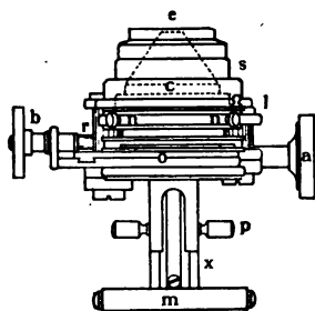
Fig. 51a. Complete Substage. Front view.
